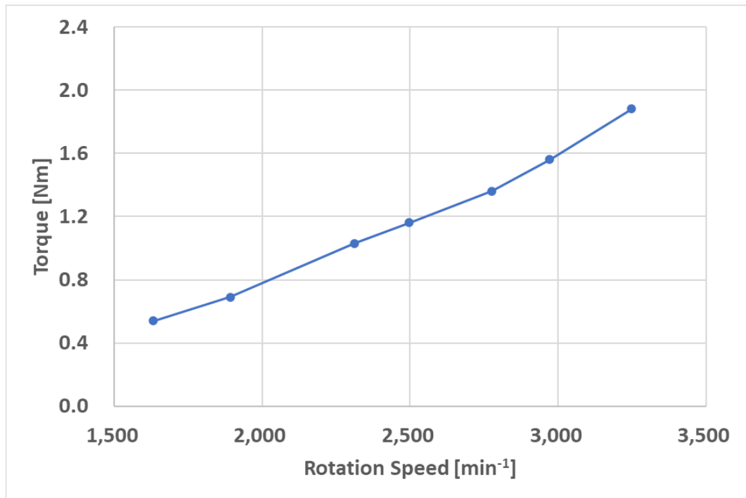
Figure 1 NT characteristics
